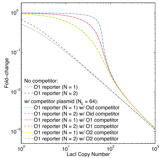
Figure S4. Comparison of Fold-Change Predictions for Multiple Chromosomal Gene Copies, Related to Figures 3 and 6
