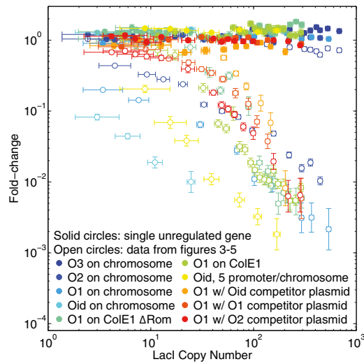
Figure S2. Comparison of Fold-Change of lacUV5 Promoter with and without Repressor Binding Site, Related to Figures 3, 4, and 5
