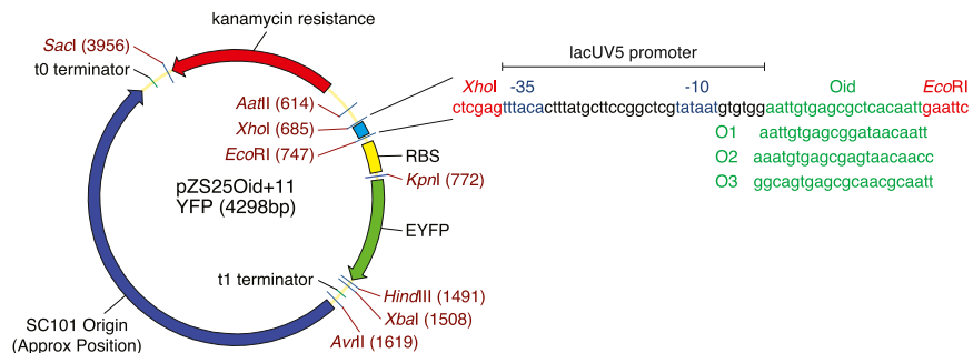
Figure S6. Plasmid Diagram and Promoter Sequence, Related to Figure 1
