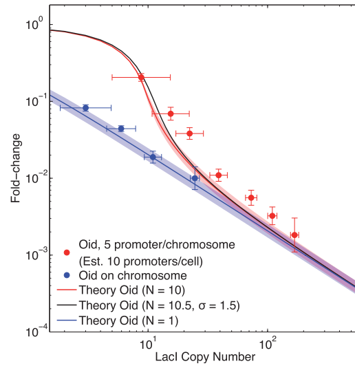
Figure S5. Effect of Copy Number Distribution on Multiple Chromosomal Integration Theory, Related to Figure 4B
