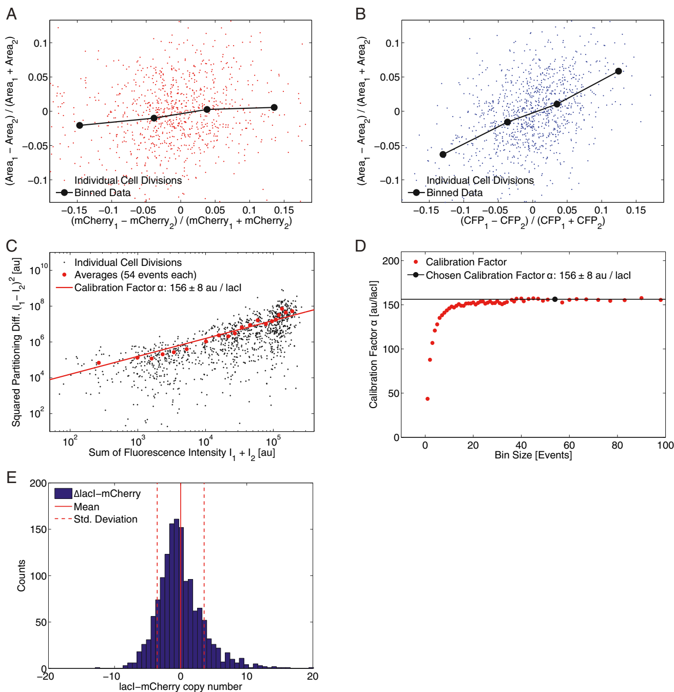
Figure S3. Determination of the Calibration Factor of LacI, Related to Figure 3
